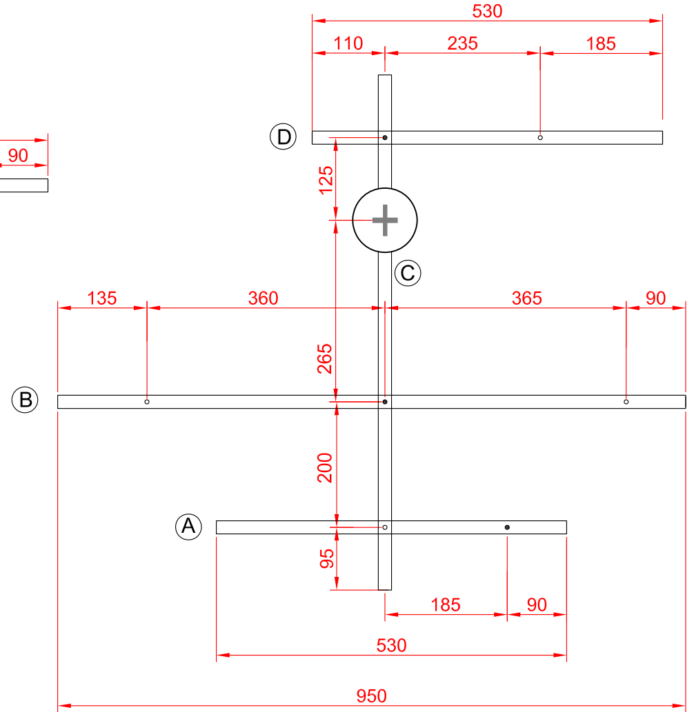
1744.178 Wall mounting-hole Distribution diagram
